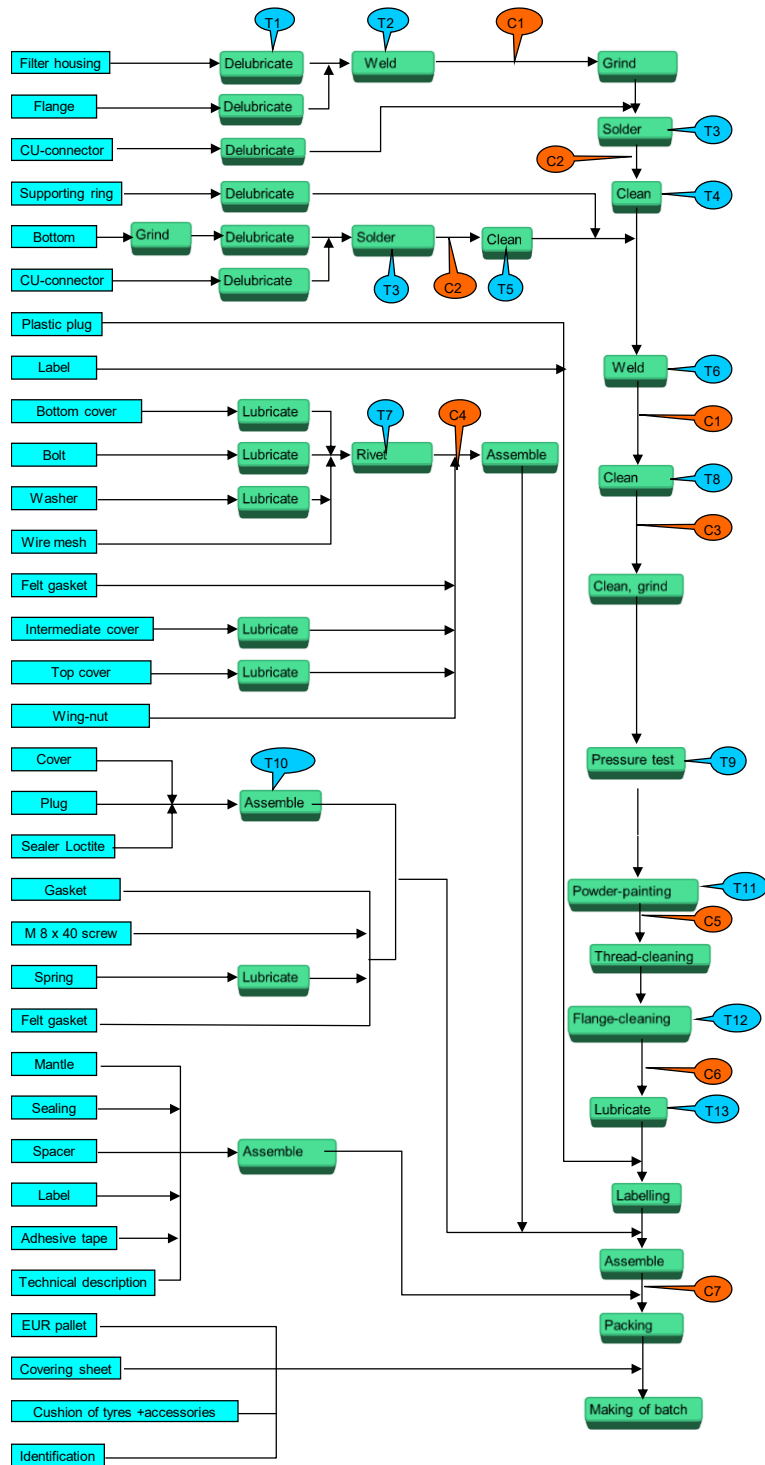
Filterhouse with CU-connector, with "2" block holder
